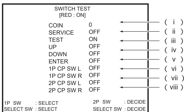
SWITCH TEST screen
